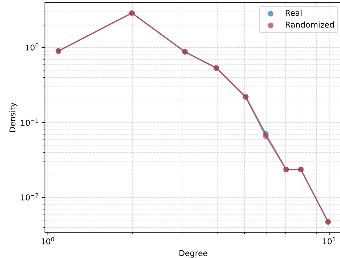
Degree distribution
